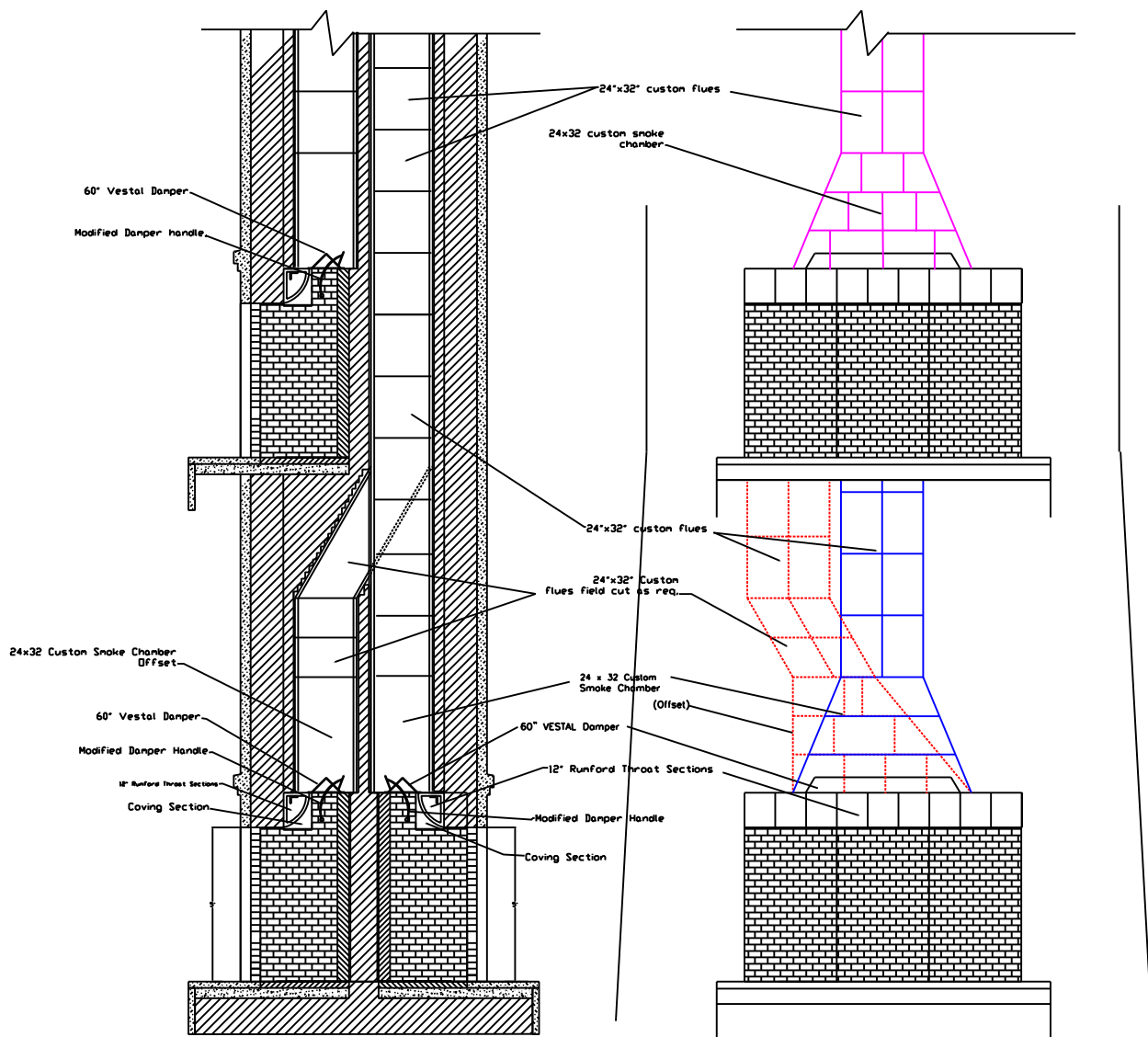
Section-Elevation
