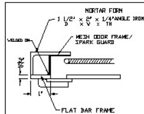
AUX. VIEW (A)
